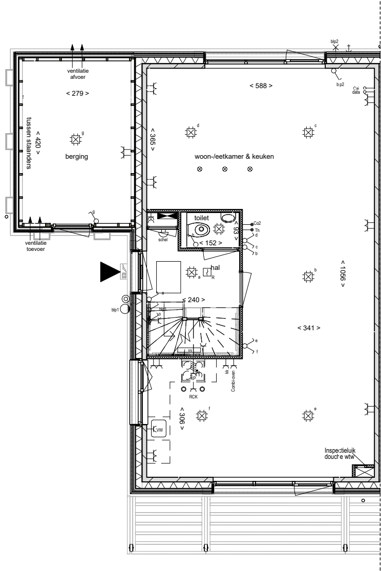
00 begane grond
